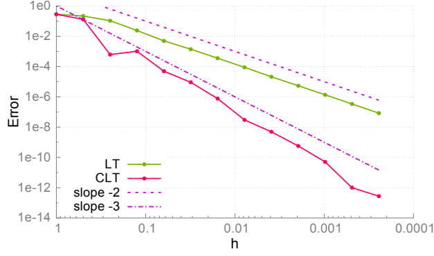
Fig. 9 Absolute error in LT and CLT for the area enclosed by the ellipse.
